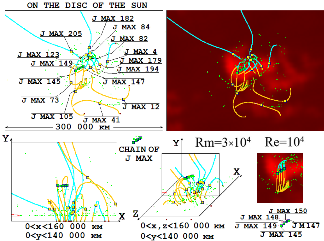
Fig. 4. Positions of current density maxima in the computation domain of the corona in space, and their projections onto the central plane of the computation domain and onto the picture plane (perpendicular to the line of sight). The distribution of microwave radio emission at a frequency of 17 GHz, obtained on the solar disk using the Nobeyama radioheliograph, is superimposed on the picture plane. The magnetic field configuration is represented by magnetic lines passing through the selected current density maxima, and their projections onto the planes. The chain of maxima consists of points marked in green.
