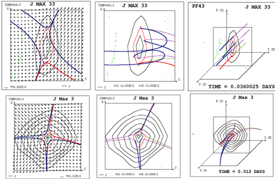
Fig. 1. Examples of magnetic field configurations in the vicinity of points on singular lines found by the graphical search system based on the results of MHD simulation.
