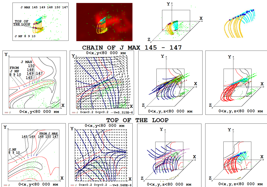
Fig. 6. Plane and spatial configurations in large regions of 80,000 km. In the central part of one of these regions there is a chain of maxima. In the central part of another region there are points at the top of an arch located on magnetic lines coming out from the points of the chain of maxima.
