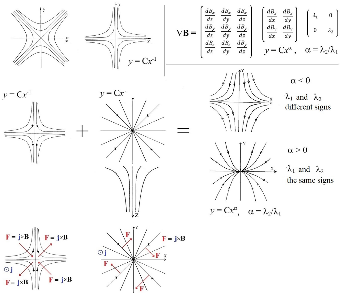
Fig. 2. Overlay of a diverging magnetic field on an X-type field in the vicinity of a singular line.
