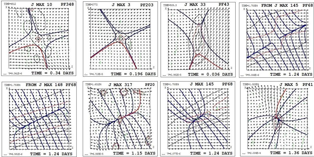
Fig. 3. Examples of plane configurations in the vicinity of singular lines, with the superposition of an X-type field and a diverging magnetic field obtained by the graphical search system based on the results of MHD simulation.
