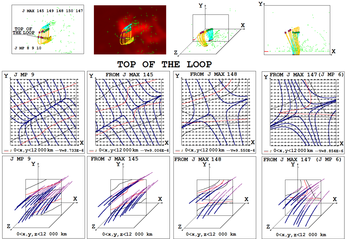
Fig. 7. Plane and spatial configurations in regions of 12,000 km in size with centers at the points at the top of the arch located on magnetic lines coming out of the points of the chain of maxima.
